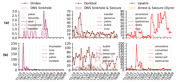
Figure 5: Relational dynamics: (a) # of SHA-2s that download target malware; and (b) # of SHA-2s dropped by target. N.B: the sharp increase in Upatre upstream droppers after mid-April, correlating with its increased use of DGA servers.
