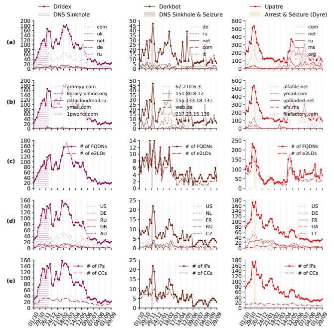
Figure 2: Aggregate network activity: (a) # of URLs used and top 5 TLDs; (b) # of URLs used and top 5 e2LDs/IPs; (c) # of FQDNs and # of e2LDs; (d) # of IPs used and top 5 hosting countries; and (e) # of IPs and # of hosting countries. Dridex exhibits consistent growth in network activity during the DNS sinkhole, while Dorkbot and Upatre both exhibit significant, short-term drops in network activity after their respective takedowns with varying long-term responses.
