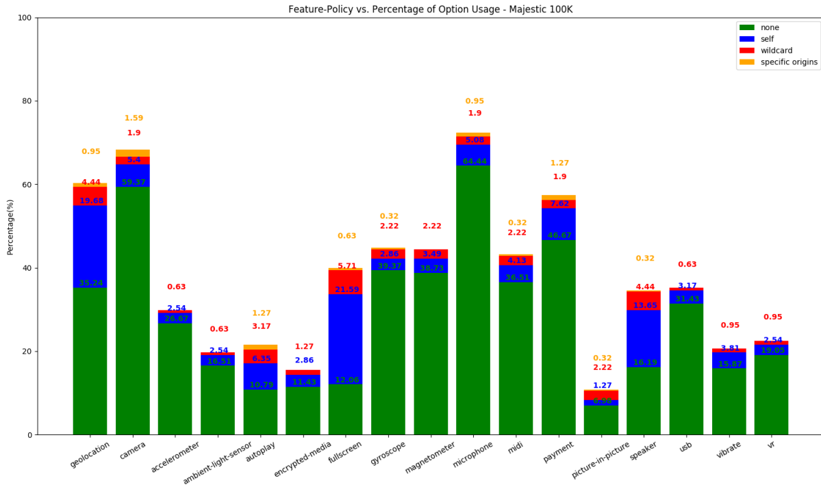
Fig. 2: Feature Policy Option Usage for Features in Majestic top 100K.
